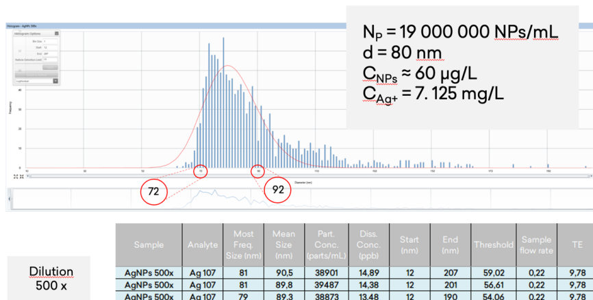
Fig. 1. Example of silver nanoparticle solution characteristics performed with SP-ICP-MS.
