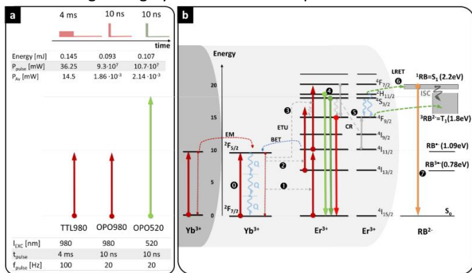
Fig. 1. The excitation schemes and mechanism of UC-LRET between \text{Yb}/\text{Er} donor NPs and Rose Bengal acceptor. (a) Three different excitation schemes used, 4 ms and 10 ns pulse and 10 ns pulse of 520 nm. (b) Energy scheme and transfer in \text{Yb}^{3+}/\text{Er}^{3+} - RB system.
