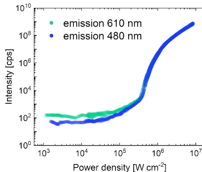
Fig.1. Luminescence intensity in a function of pump power density for sample NaYF 4 :0.5%Pr 3+ ,15%Yb 3+ @NaYF 4
