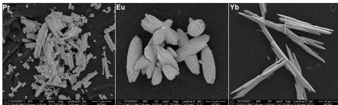
Fig. 1. SEM micrographs of \text{Pr}_4\text{O}_3\text{F}_6 (left), \text{Eu}_4\text{F}_3\text{O}_6 (center) and \text{Yb}_4\text{F}_3\text{O}_6 (right).
